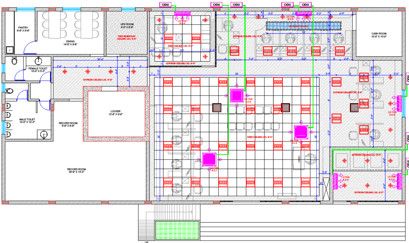
FALSE CEILING LAYOUT
